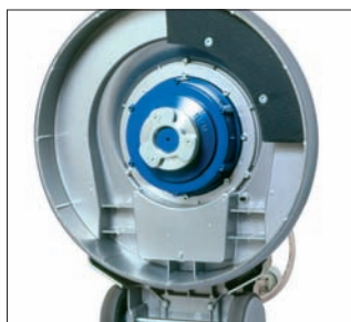
Attacco disco trascinatore e spazzole Mount for drive board and brushes
